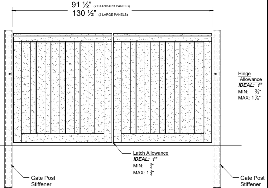
DOUBLE GATE OPENING
